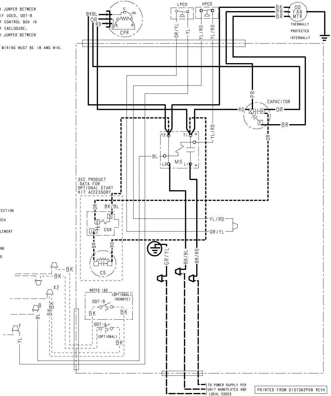
Figure 2. 018, 019, 024, 025, 042 & 049 Models
