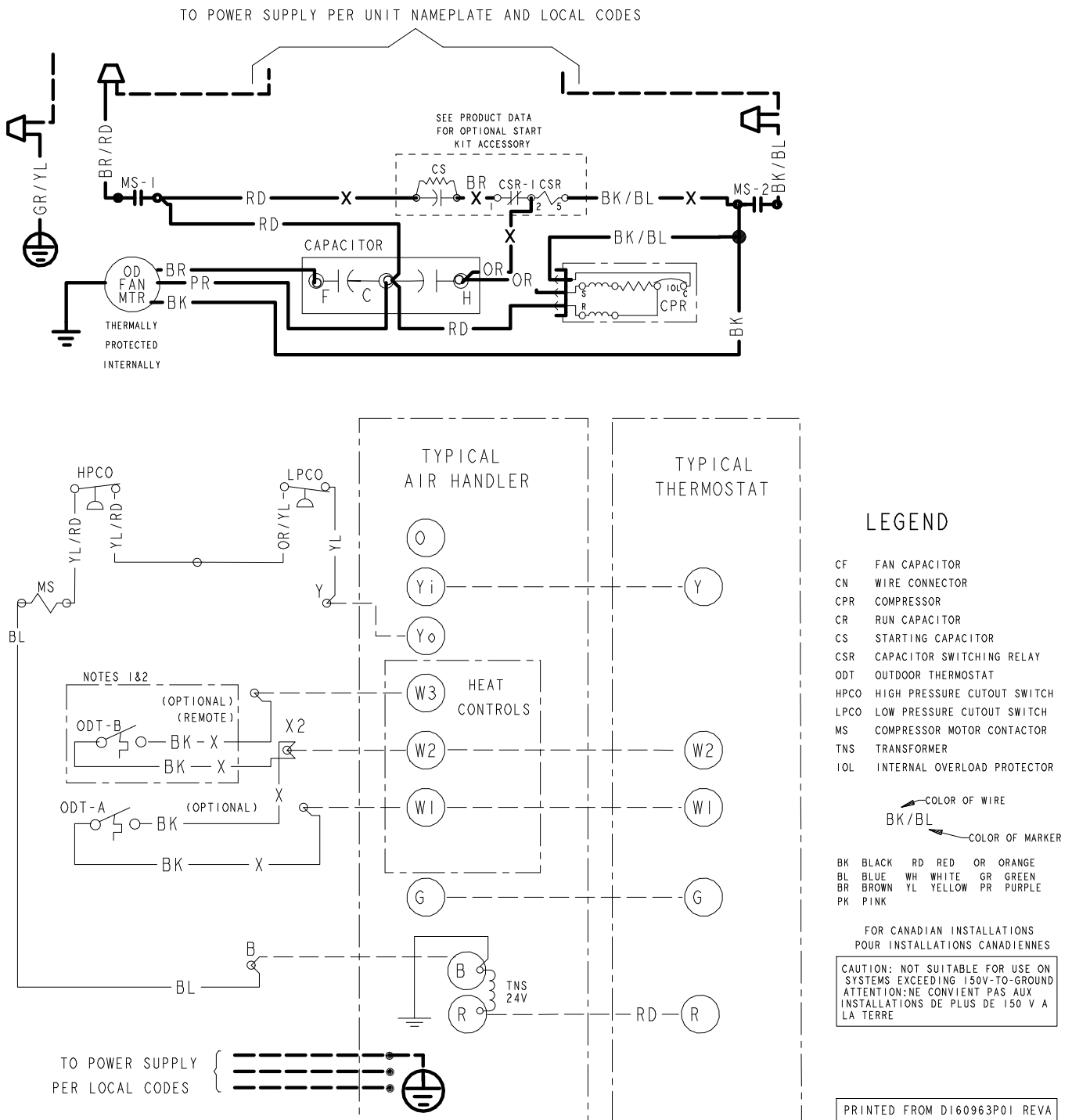
Figure 5. 060 Models
