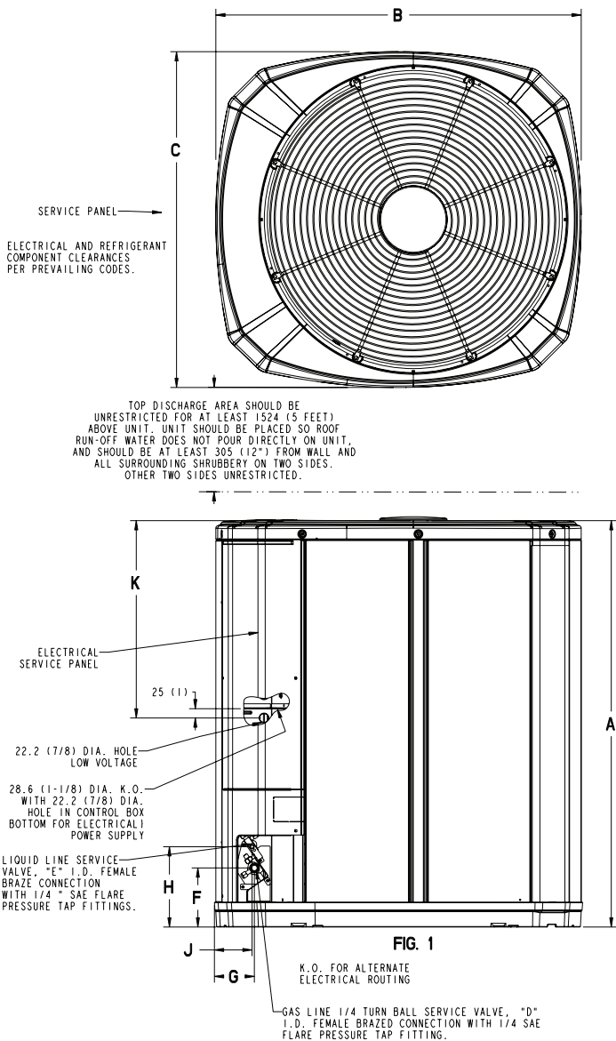
From Dwg. D152862 Rev. 21
