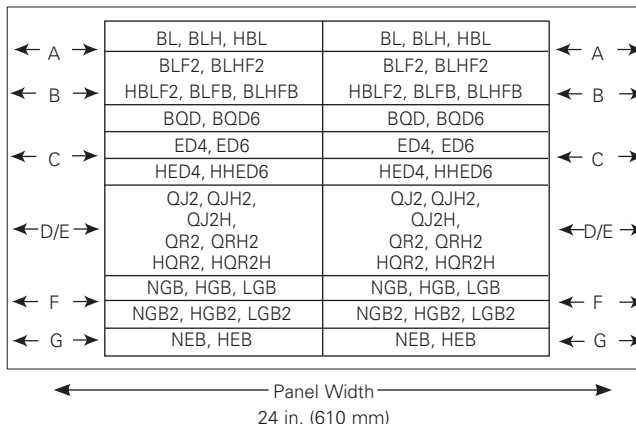
Branch Breaker Side Gutters
