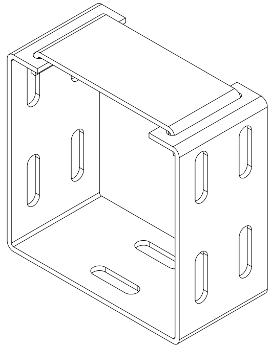
ISOMETRIC VIEW
