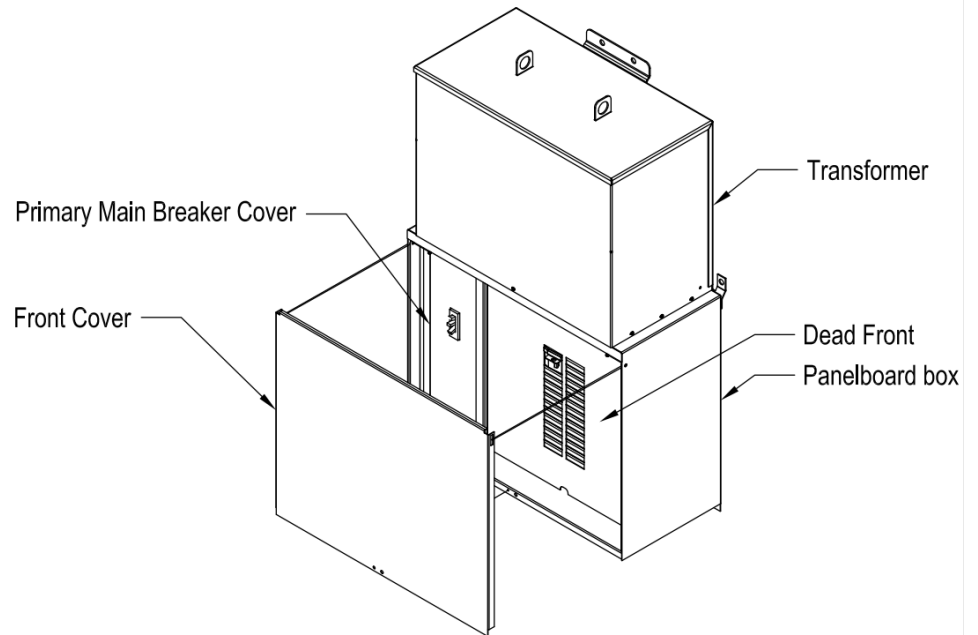
Figure 15 - Exploded parts
