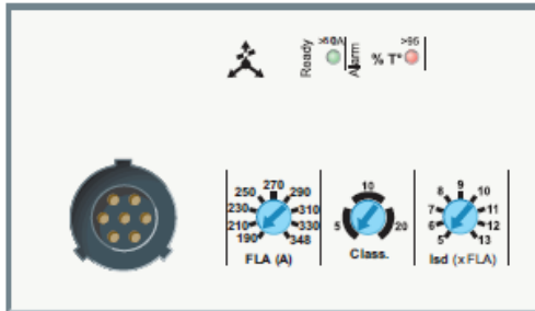
MicroLogic 2.2M and 2.3M Trip Units
