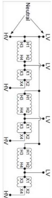
Wiring Diagram 7
