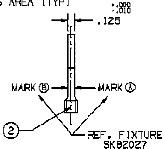
SECTION A-A TYPICAL
