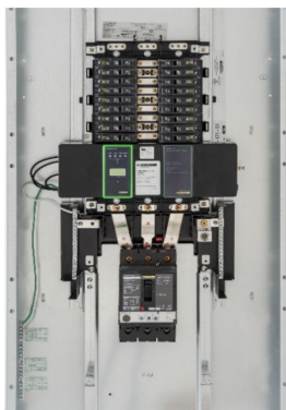
NQ Main Circuit Breaker Interior with SurgeLoc™ SPD
