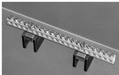
Ground Bar with Insulator Kit
