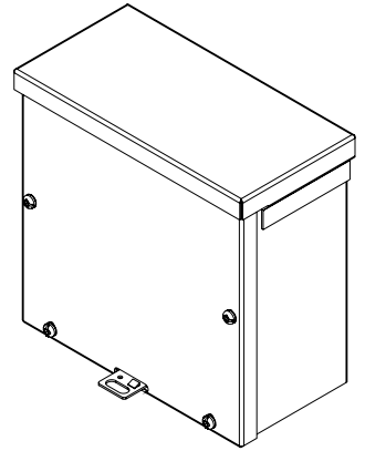
ISOMETRIC VIEW
