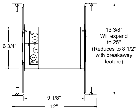
4 1/2" CEILING CUTOUT
