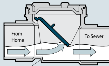
Built-in drainage slope
