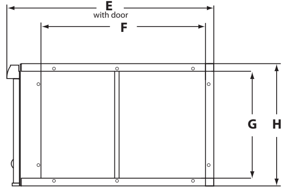
Inlet Side Return Duct Connection
