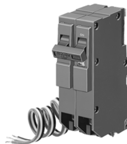
QO-PL 2-Pole
